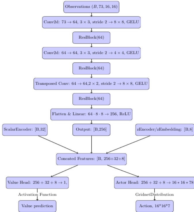
Figure 4. The Network Architecture
