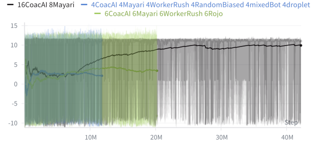
Figure 7. Episode rewards (y-axis) as a function of training timesteps (x-axis) on the BC-FT agent.
