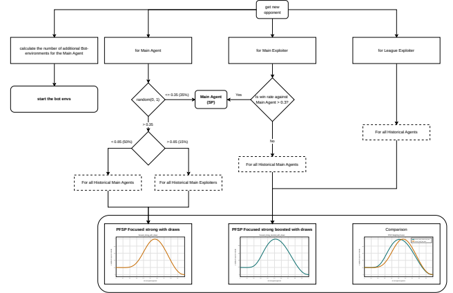
Figure 5. Matchmaking process for the league. Dashed boxes are candidate opponent sets, while the percentages on the arrows are fixed sampling probabilities. The PFSP curve gives the weighting for the opponent win rate
