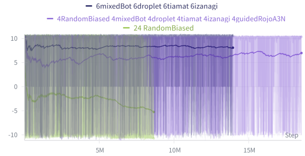
Figure 8. Episode rewards (y-axis) as a function of training timesteps (x-axis) on the final agent.
