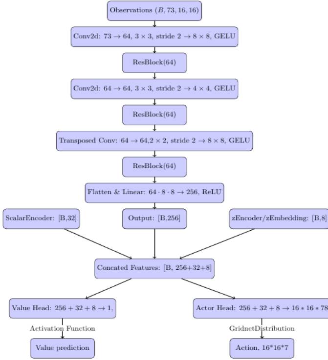
Figure 6. The Network Architecture
