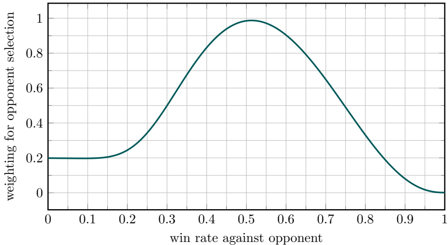
focused_strong_boosted_with_draws
