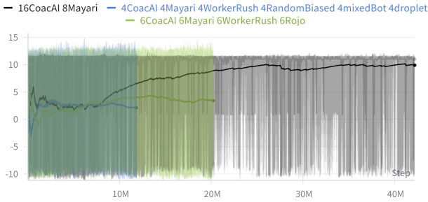
Figure 6. Episode rewards (y-axis) as a function of training timesteps (x-axis) on the BC-FT agent.
