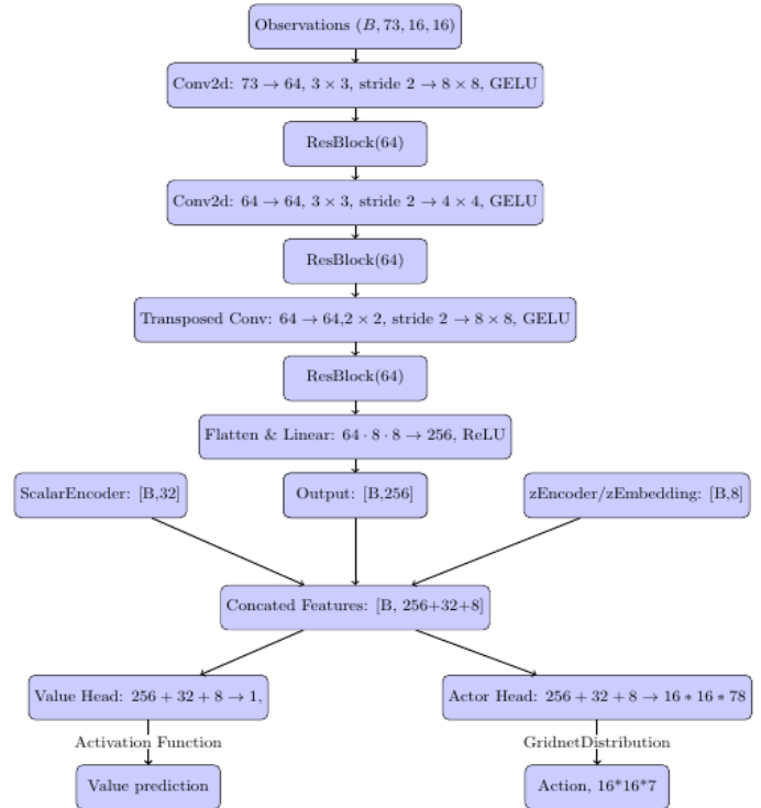
Figure 5. The Network Architecture
