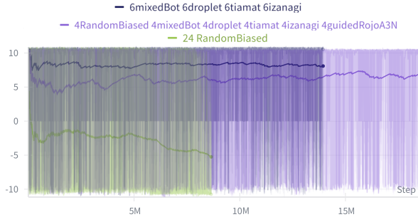
Figure 7. Episode rewards (y-axis) as a function of training timesteps (x-axis) on the final agent.
