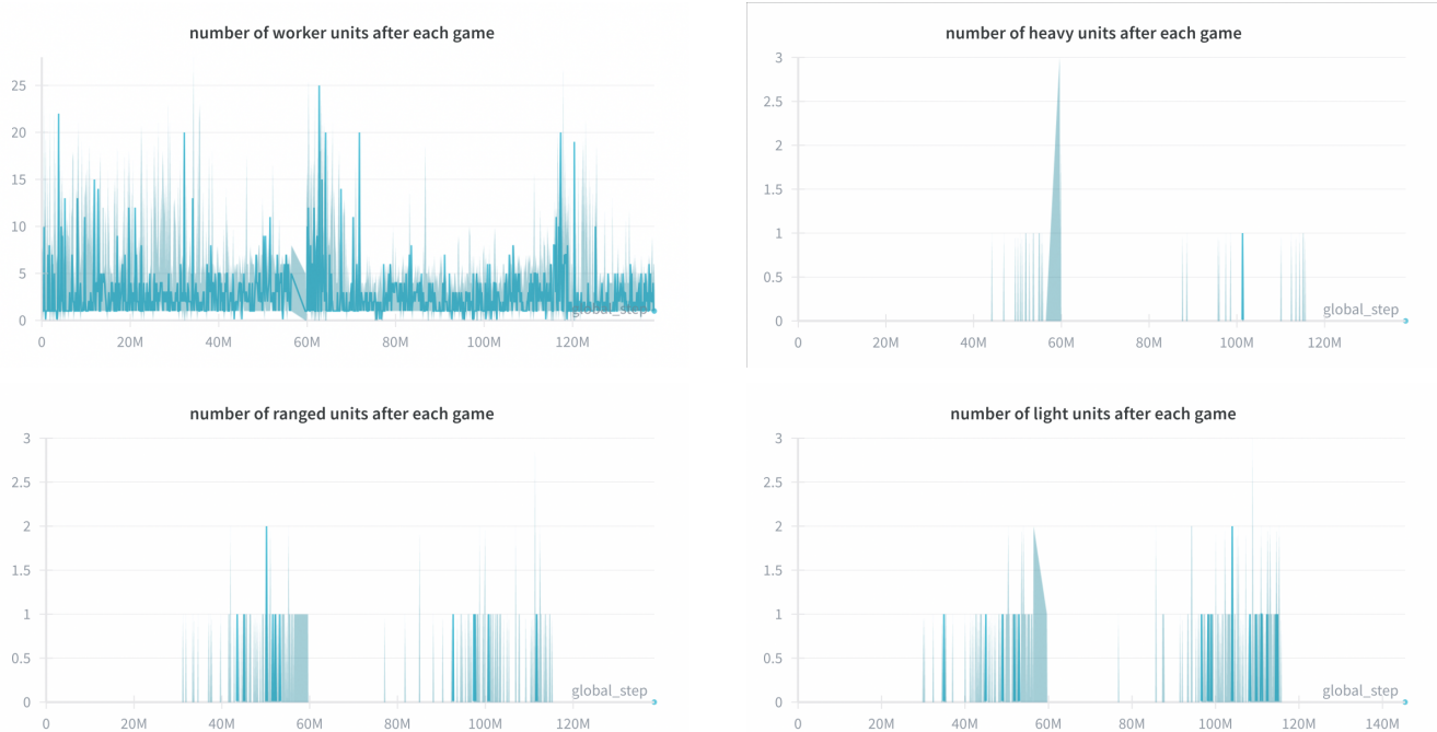
Figure 5. Number of units after each game for the agents initialized with worker focused (shown are 2 full reset cycles).
