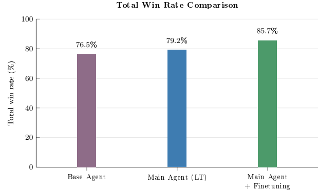
Figure 1. Comparison of total win rates for the Base Agent, the Main Agent after LT and the Main Agent after finetuning against all our evaluation opponents.
