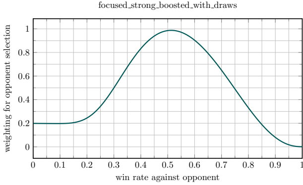
Figure 5. Prioritization function for the Main Agent in PFSP.
