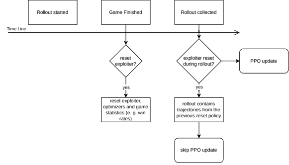
Figure 6. When resetting exploiters skip the update for the current rollout.
