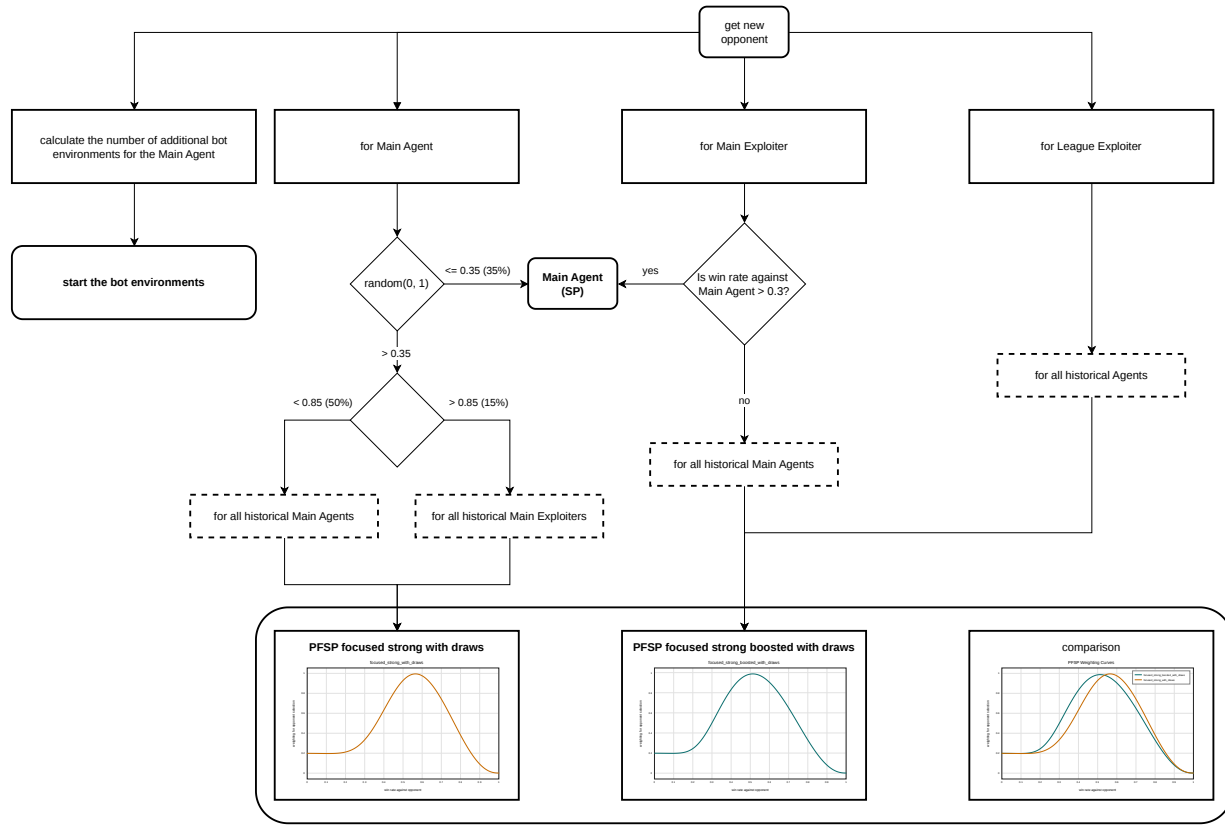
Figure 5. Matchmaking process for LT. Dashed boxes are candidate opponent sets, while the percentages on the arrows are fixed sampling probabilities. The PFSP curve gives the weighting for the opponent win rate.
