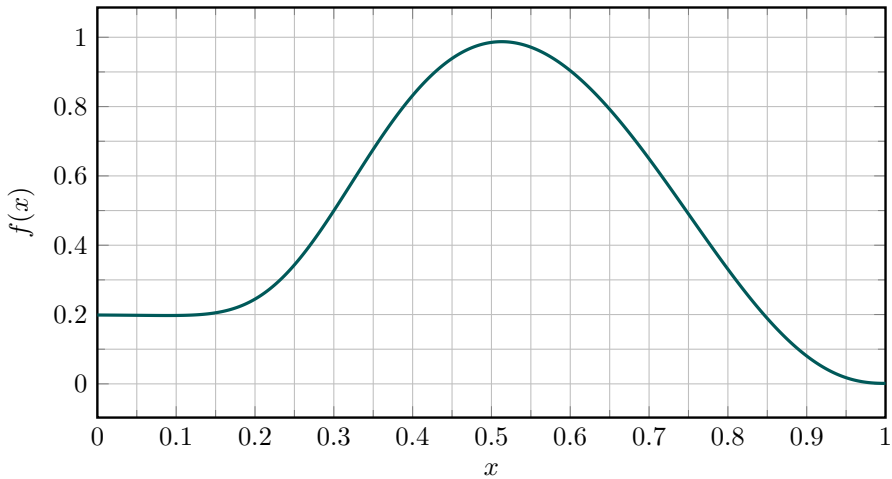
focused_strong_boosted_with_draws
