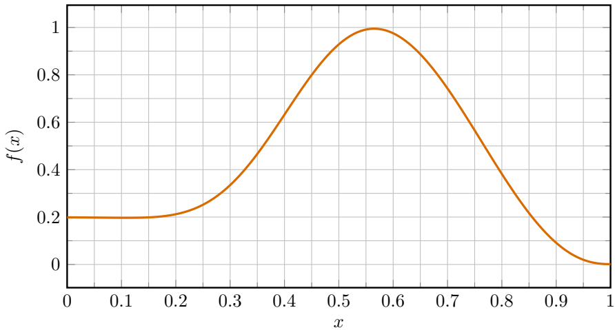
focused_strong_with_draws
