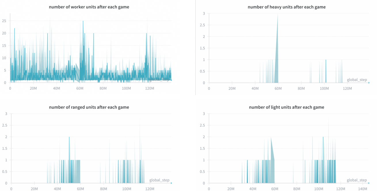
Figure 5. Number of units after each game for the agents initialized with Worker focused (shown are 2 full reset cycles).
