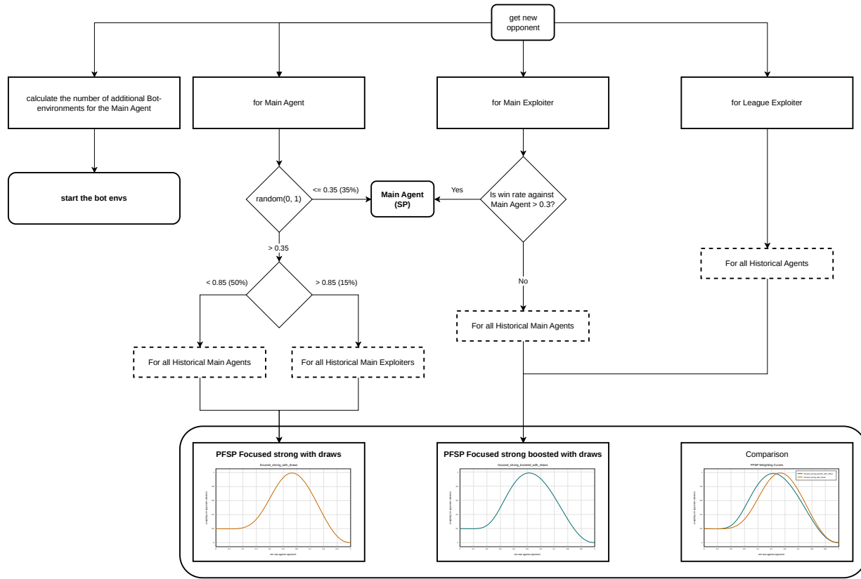
Figure 6. Matchmaking process for the league. Dashed boxes are candidate opponent sets, while the percentages on the arrows are fixed sampling probabilities. The PFSP curve gives the weighting for the opponent win rate
