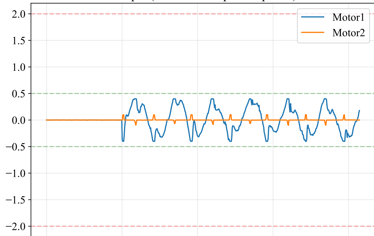
Torque (Utilization Opt / Proposed)
