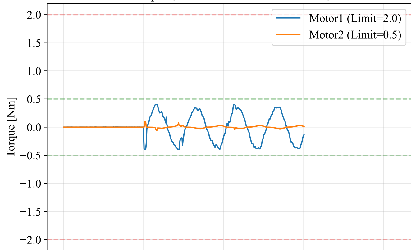
Torque (Fixed Ratio / Conventional)
