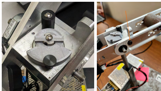
Figure 8-2: Close-up images of the two screws used to restrict yaw (shown on left) and pitch (shown on right). Make sure the screws are centered and well-seated.
