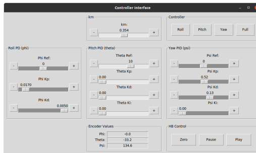
Figure 10-1: GUI used for lab H.10
