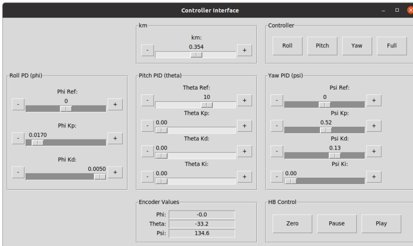
Figure 7-3: Screen-shot of the hummingbird GUI in “pitch” control mode.
