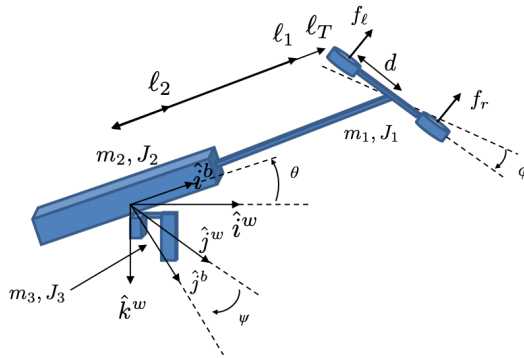
Figure 1-1: Hummingbird coordinate frames and nomenclature.
