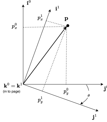
Figure 2-2: Rotation in 2D
