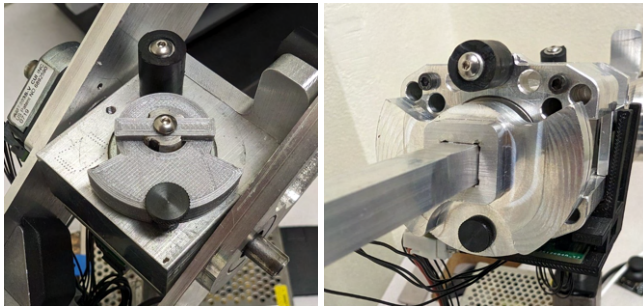
Figure 4-1: For this lab, we will only use the “pitch” degree of freedom ( \theta ). Close-up images of the two screws used to restrict yaw (shown on left) and roll (shown on right) are shown. Make sure the screws are centered and well-seated.
