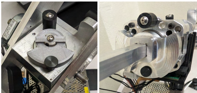
Figure 7-2: Close-up images of the two screws used to restrict yaw (shown on left) and roll (shown on right). Make sure the screws are centered and well-seated.
