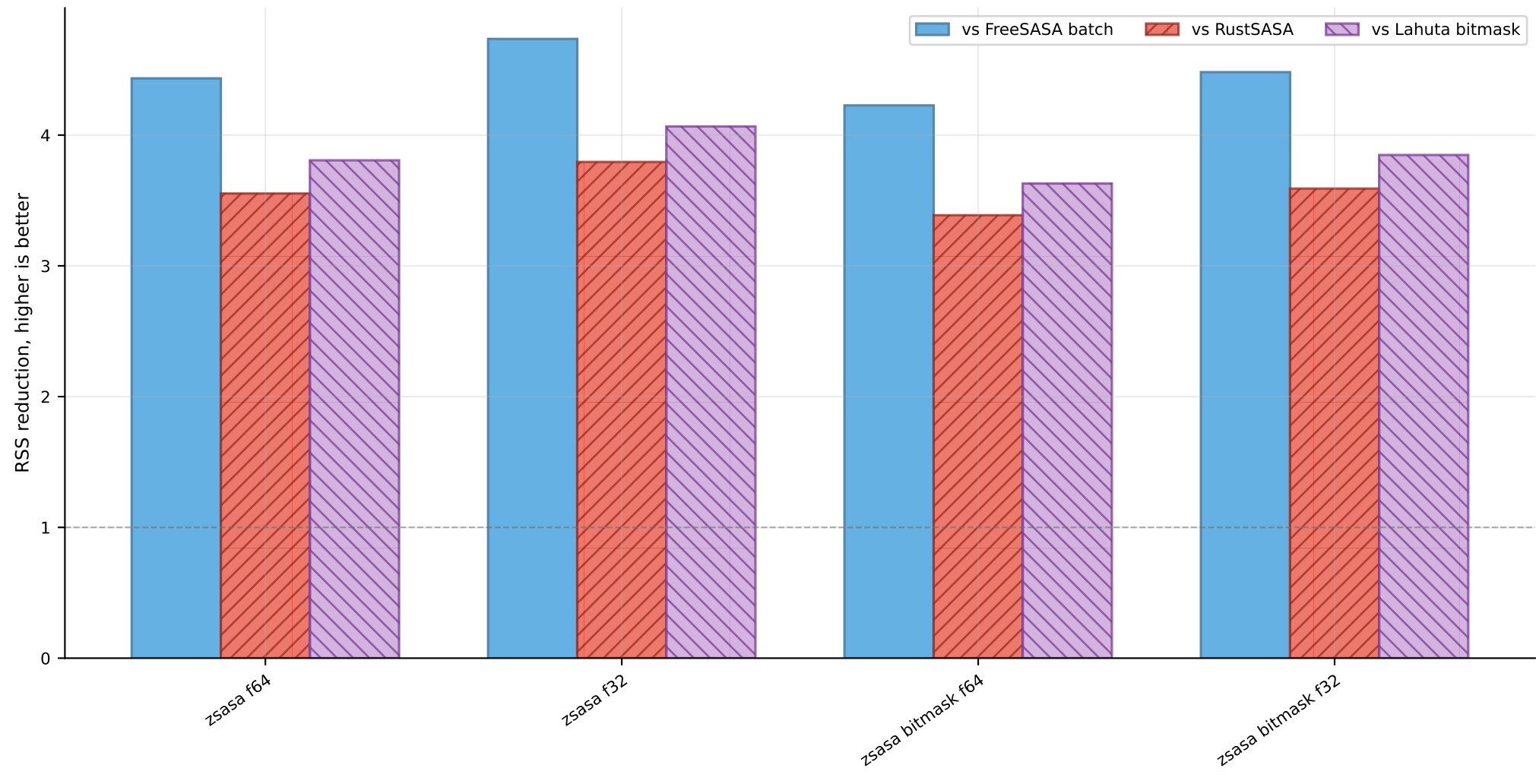
E. coli batch RSS reduction: zsasa vs FreeSASA/RustSASA/Lahuta bitmask at 10 threads
