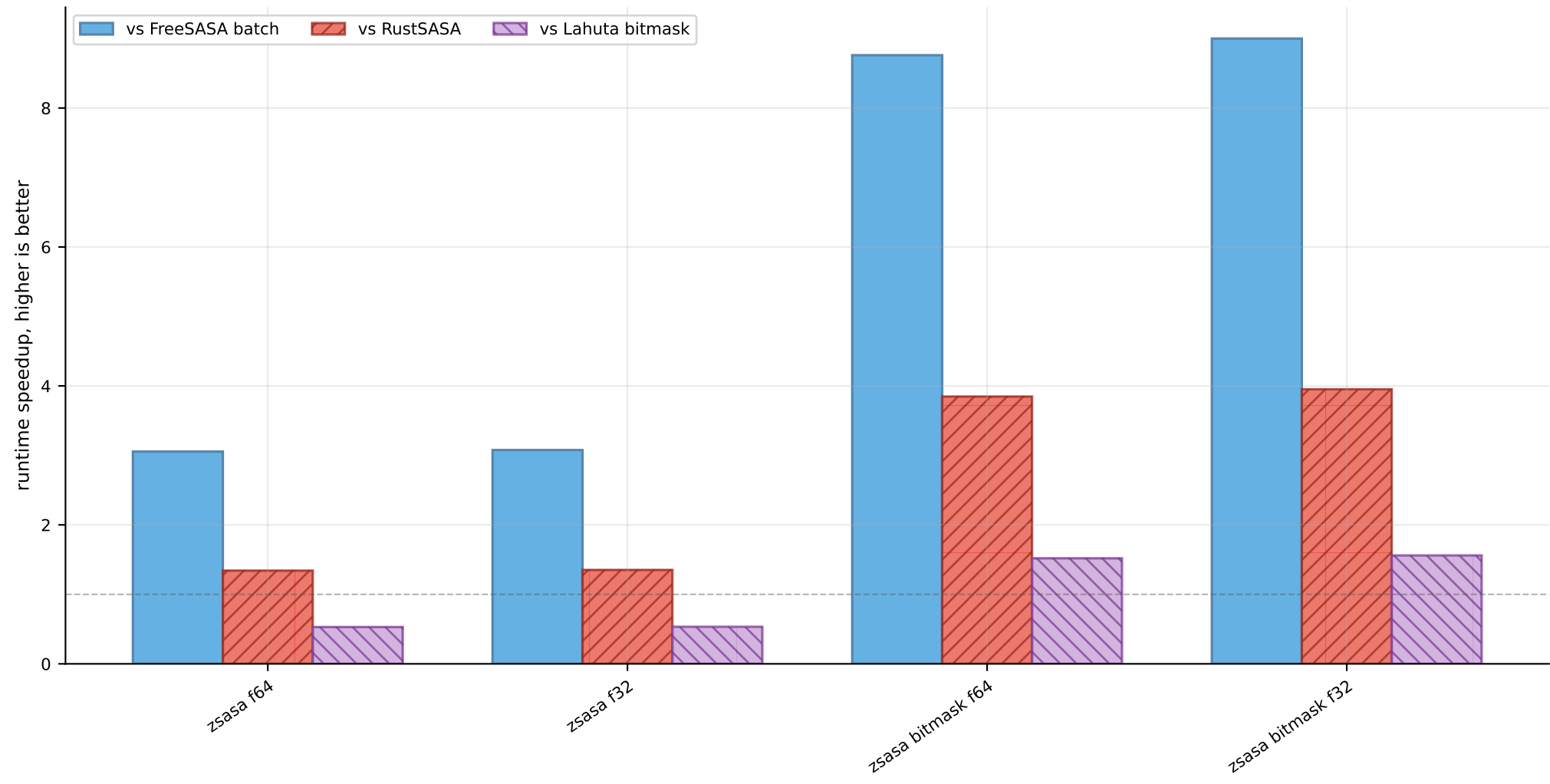
E. coli batch runtime speedup: zsasa vs FreeSASA/RustSASA/Lahuta bitmask at 10 threads
