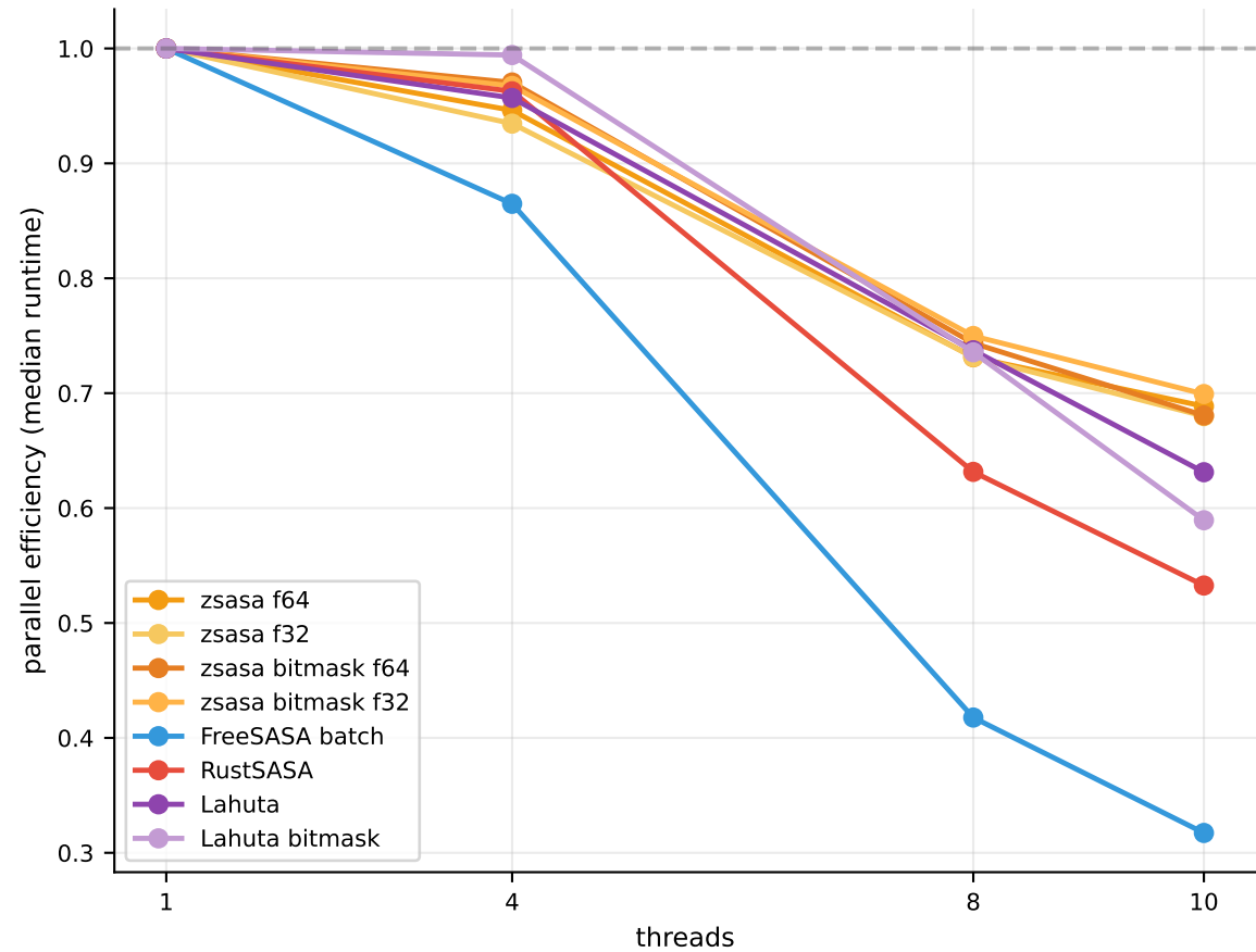
Thread efficiency
