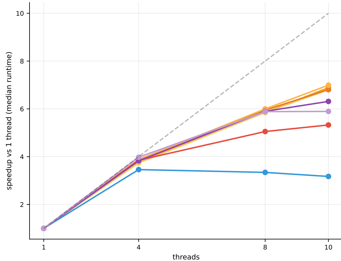
Thread speedup
