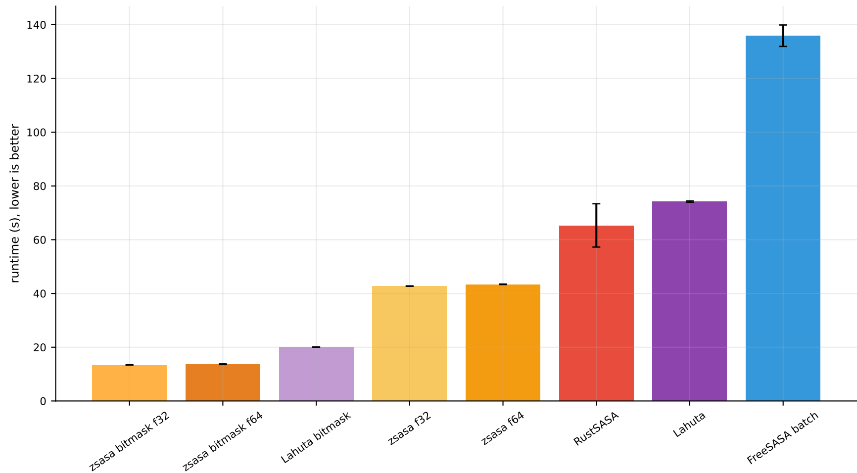
Human batch runtime at 10 threads
