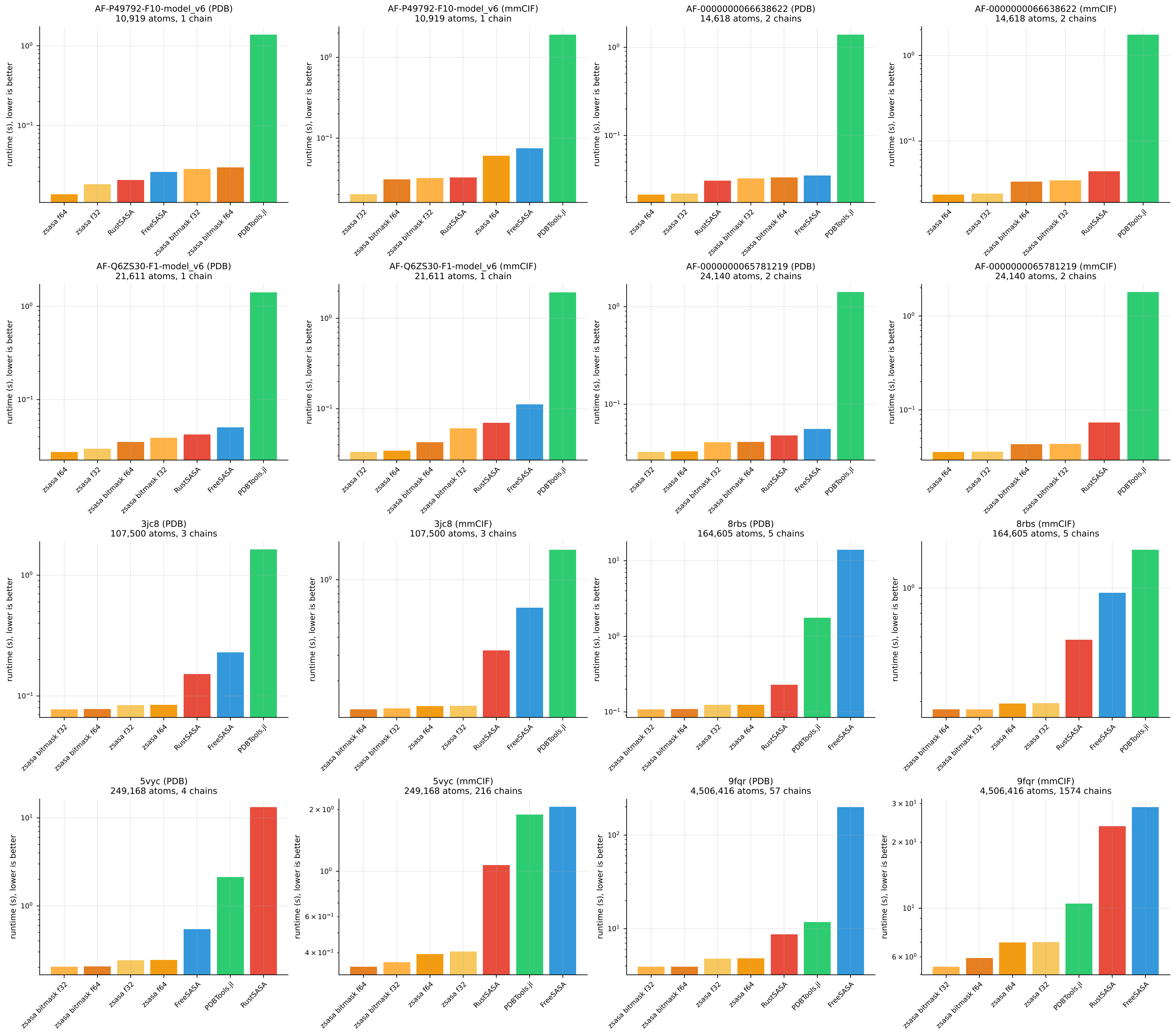
Single-file runtime at 10 threads
