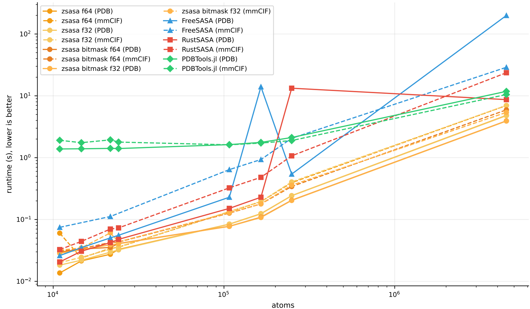
Single-file runtime vs atoms at 10 threads
