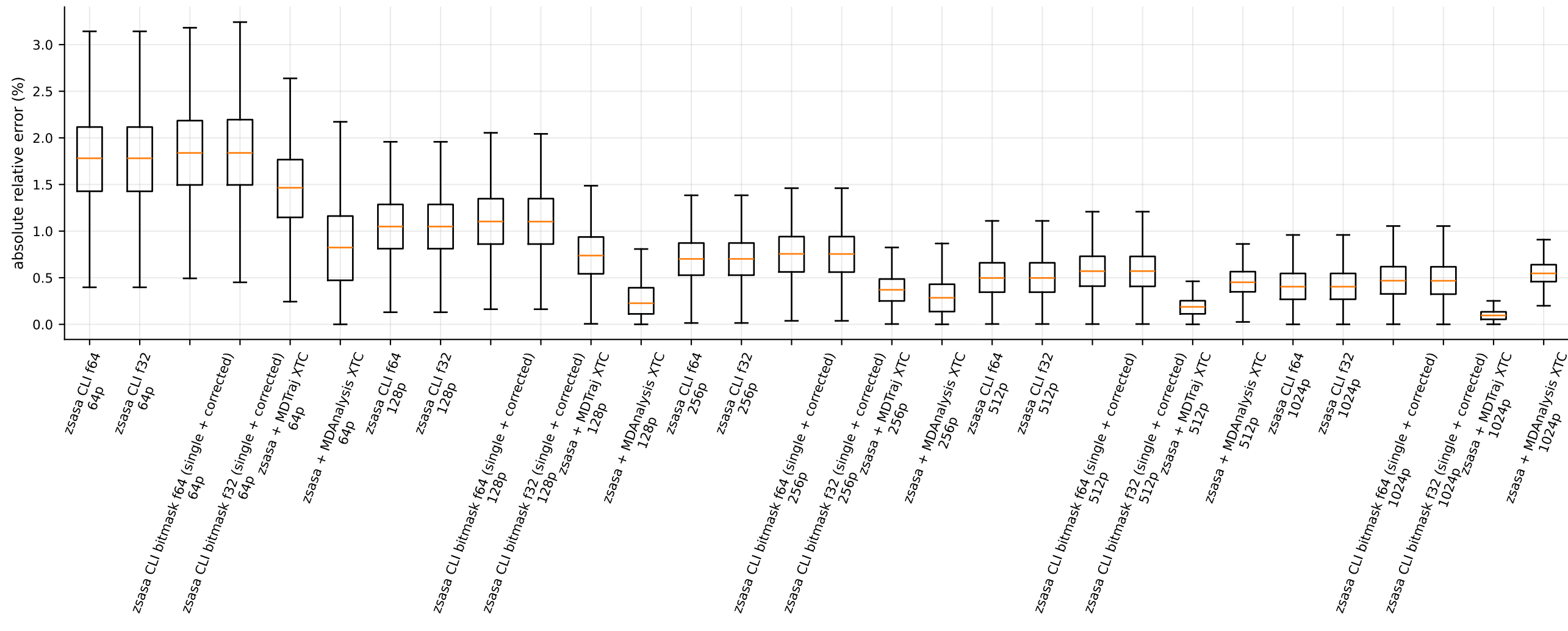
MD validation error distributions
