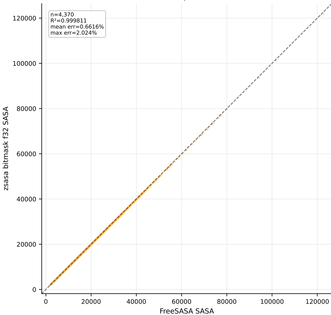
zsasa bitmask f32 128 points
