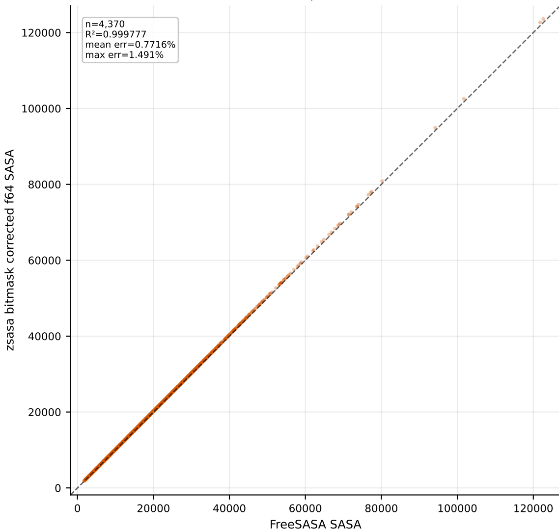
zsasa bitmask corrected f64 512 points
