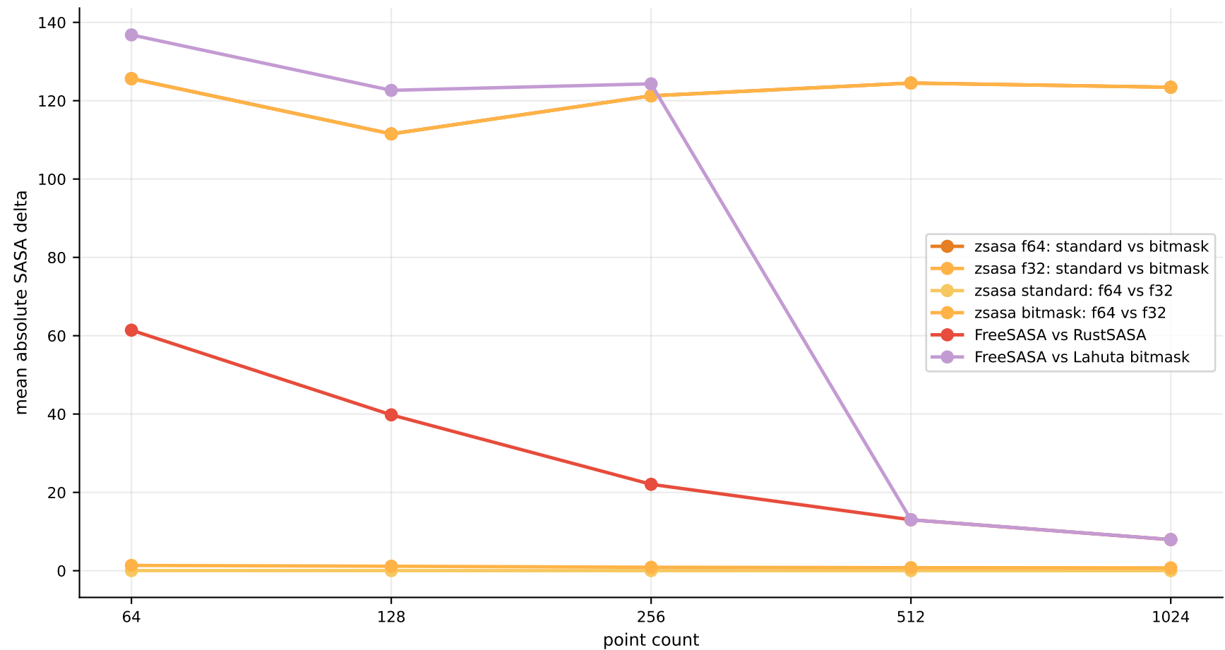
Static SR validation variant deltas
