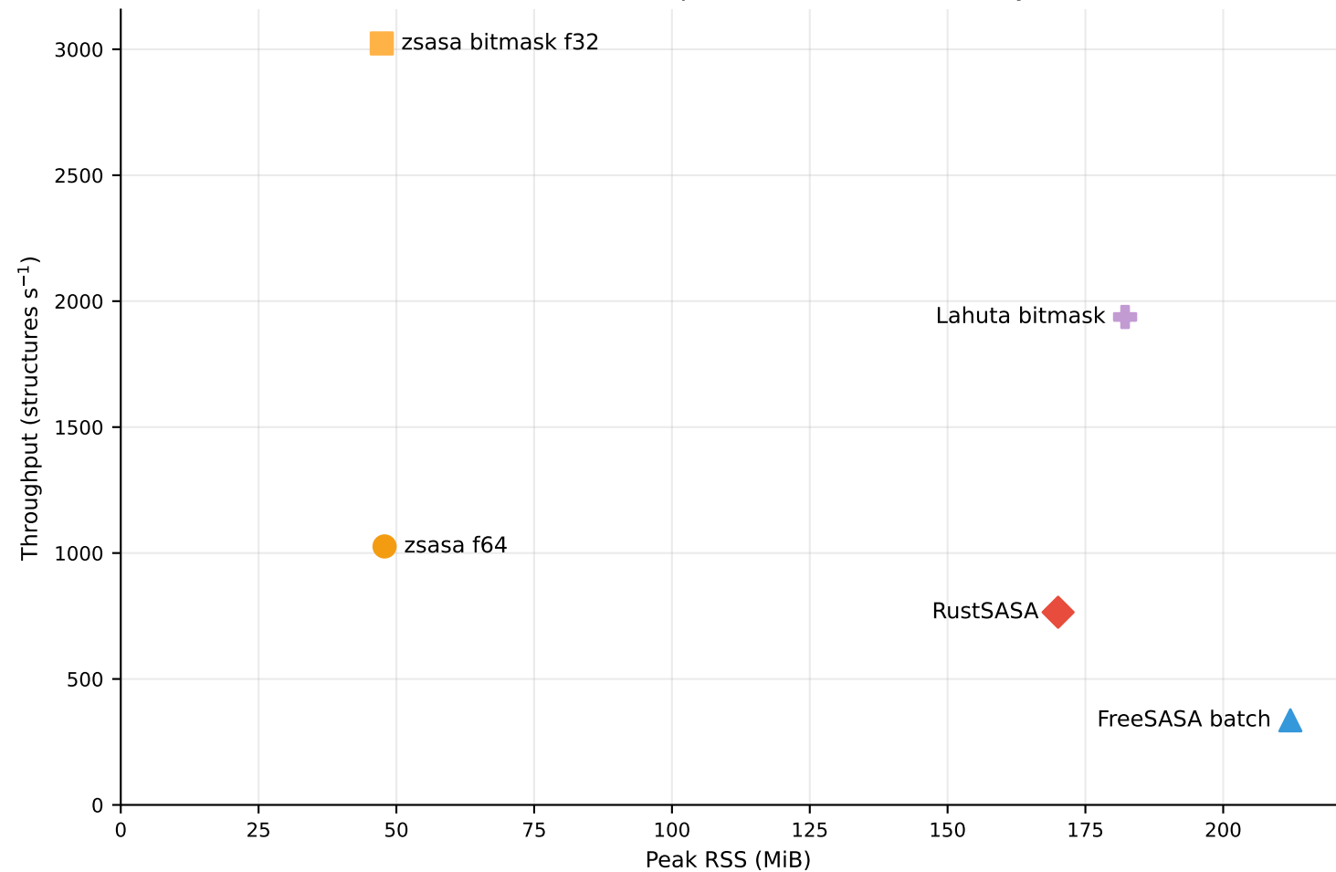
E. coli AFDB batch performance and memory
