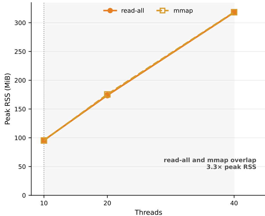
Memory cost
