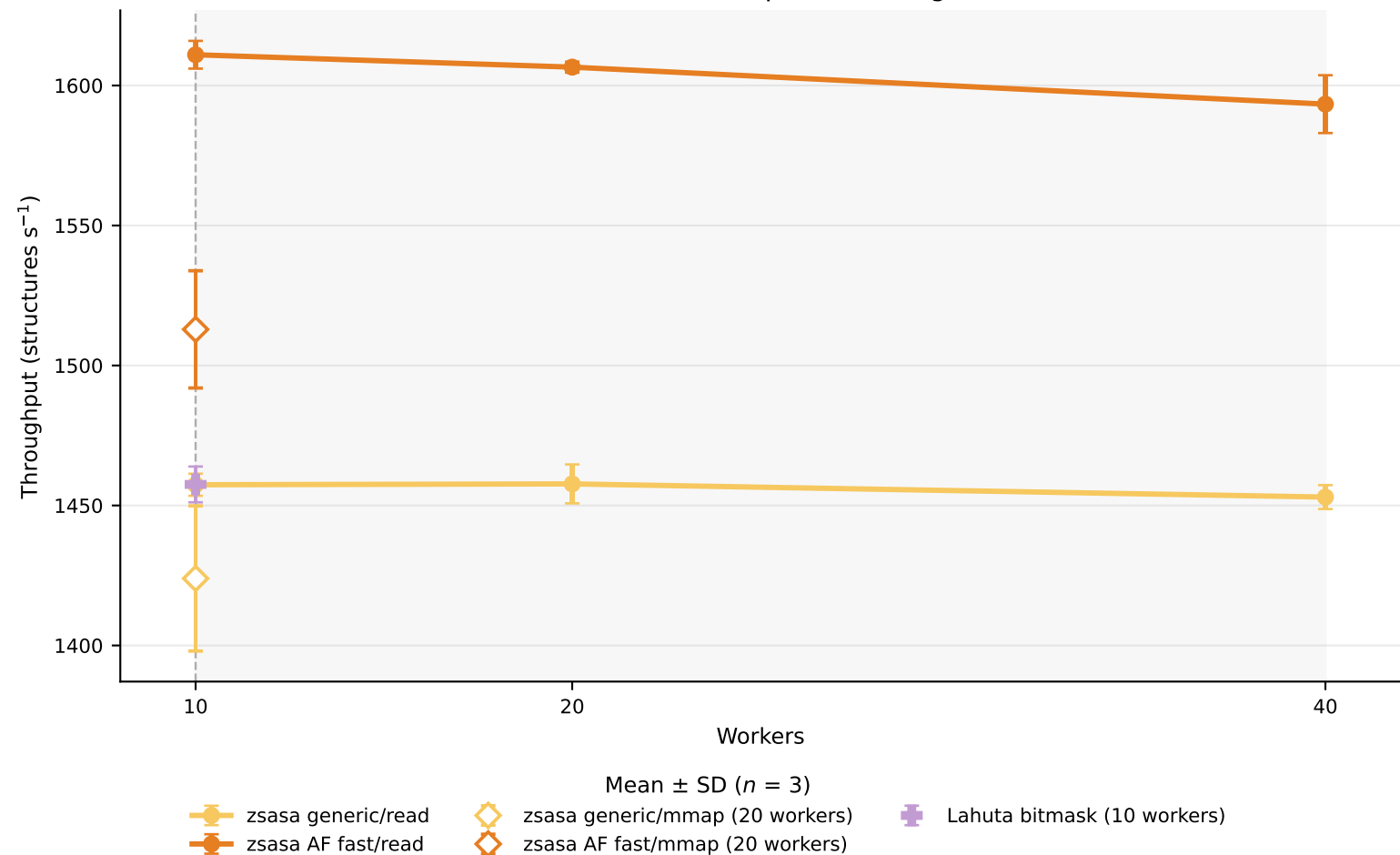
Human AFDB mmCIF batch throughput by worker count (23,586 structures, 128 points, 10 logical CPUs)
