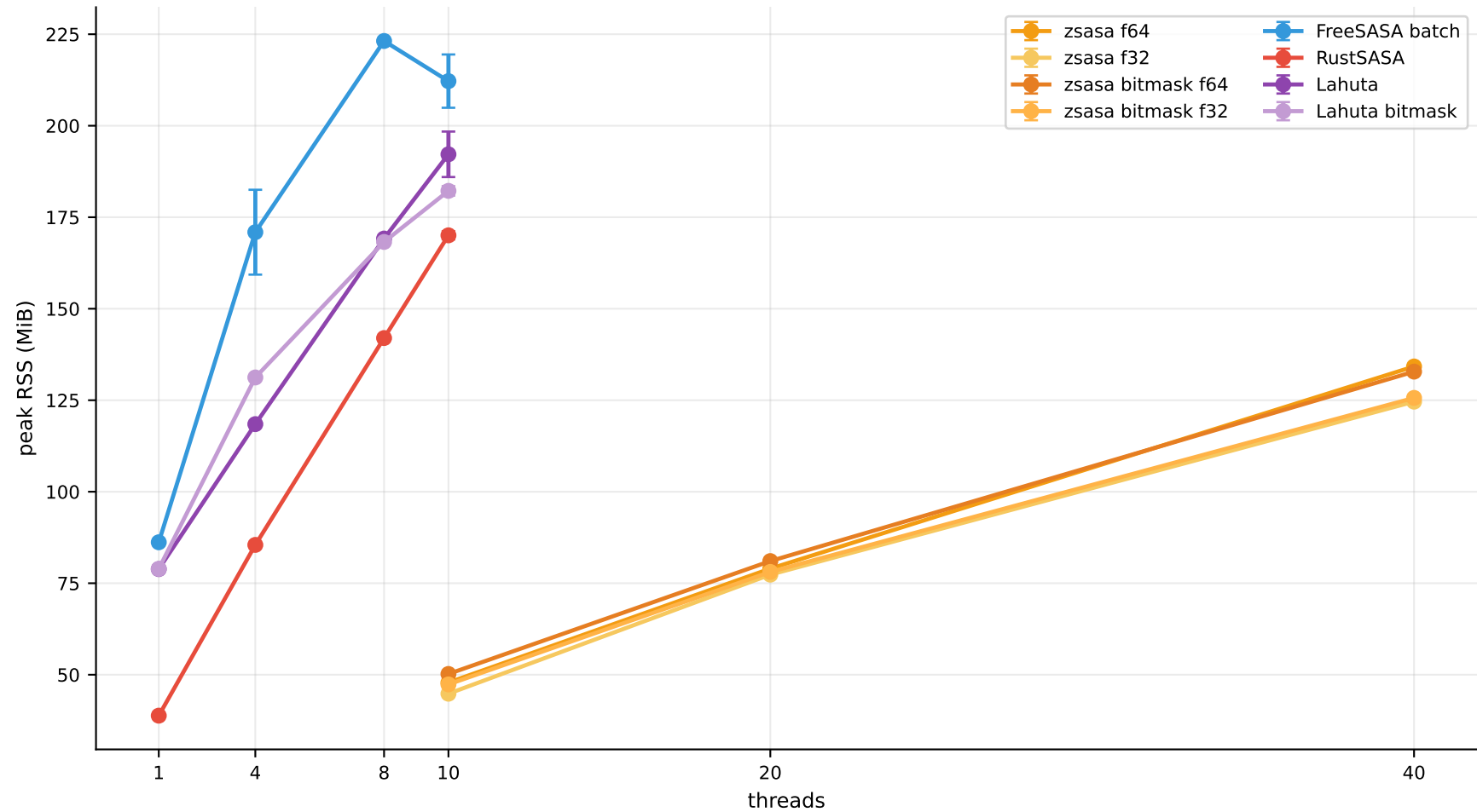
E. coli batch peak RSS
