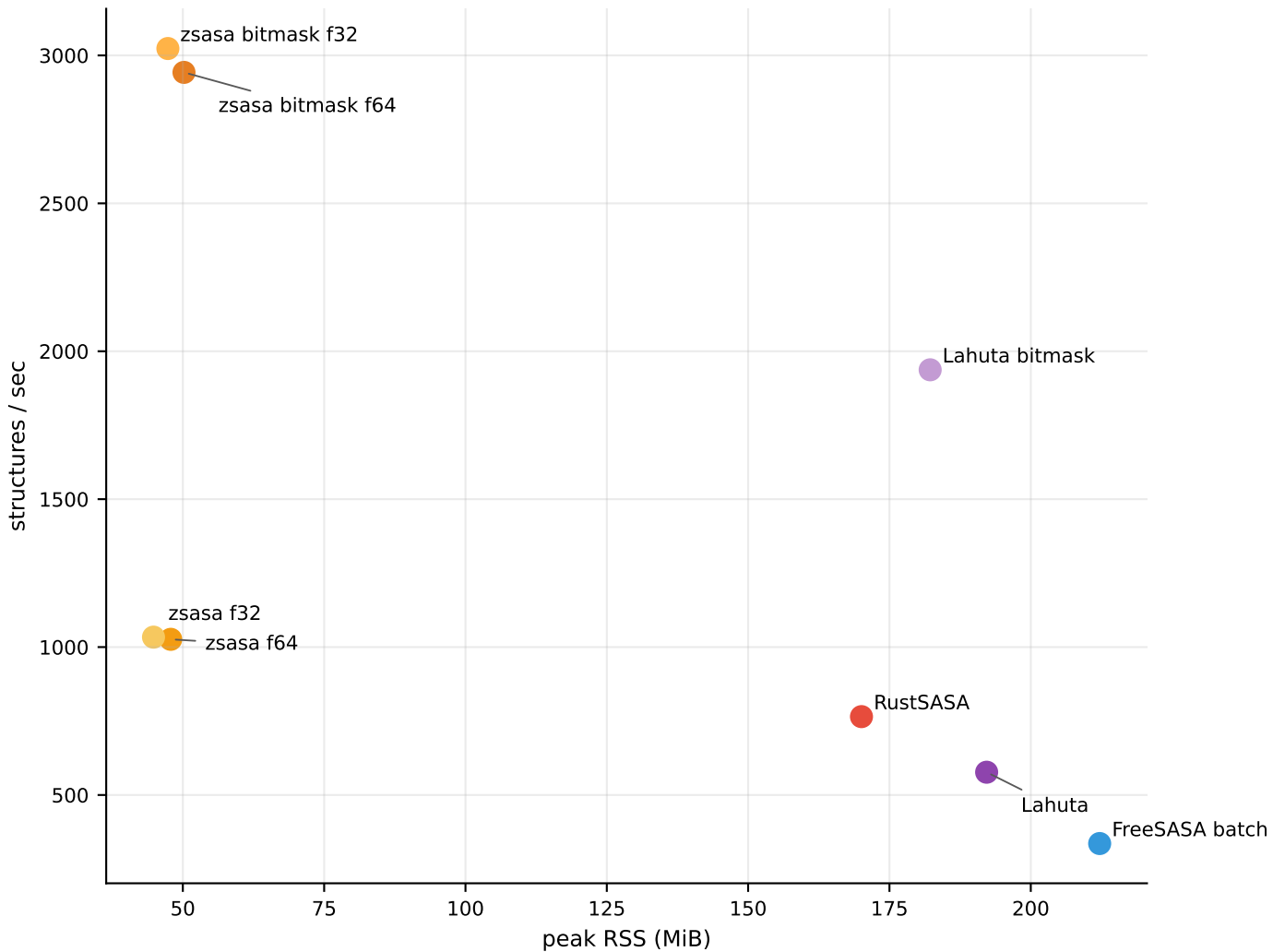
E. coli batch throughput vs peak RSS at 10 threads
