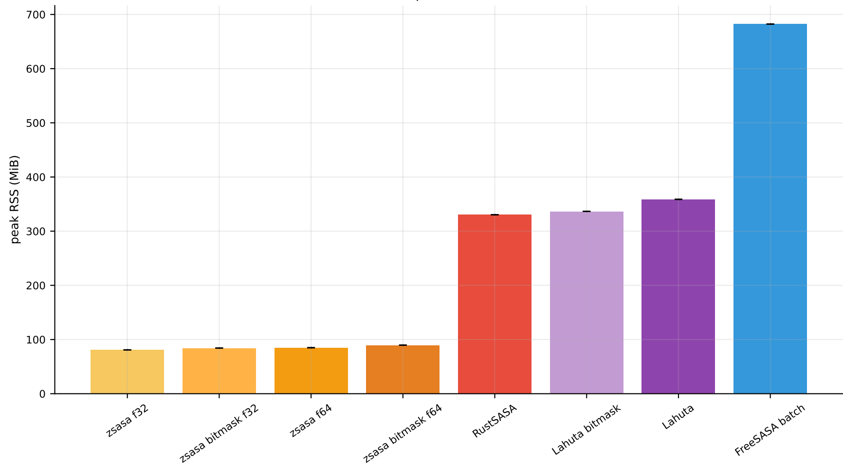
Human batch peak RSS at 10 threads
