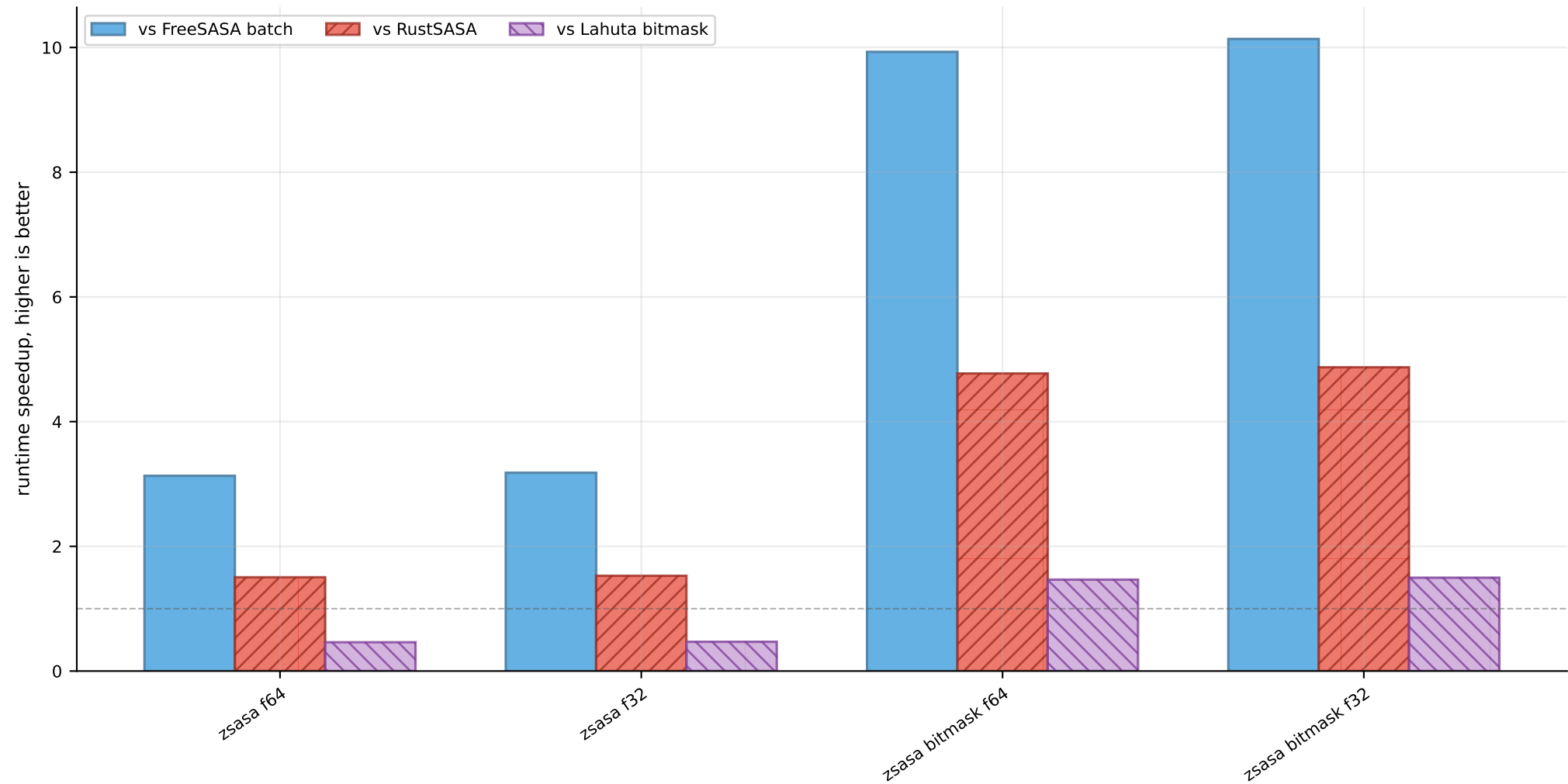
Human batch runtime speedup: zsasa vs FreeSASA/RustSASA/Lahuta bitmask at 10 threads
