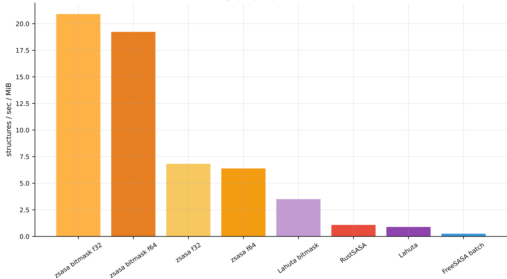
Human throughput per peak RSS at 10 threads
