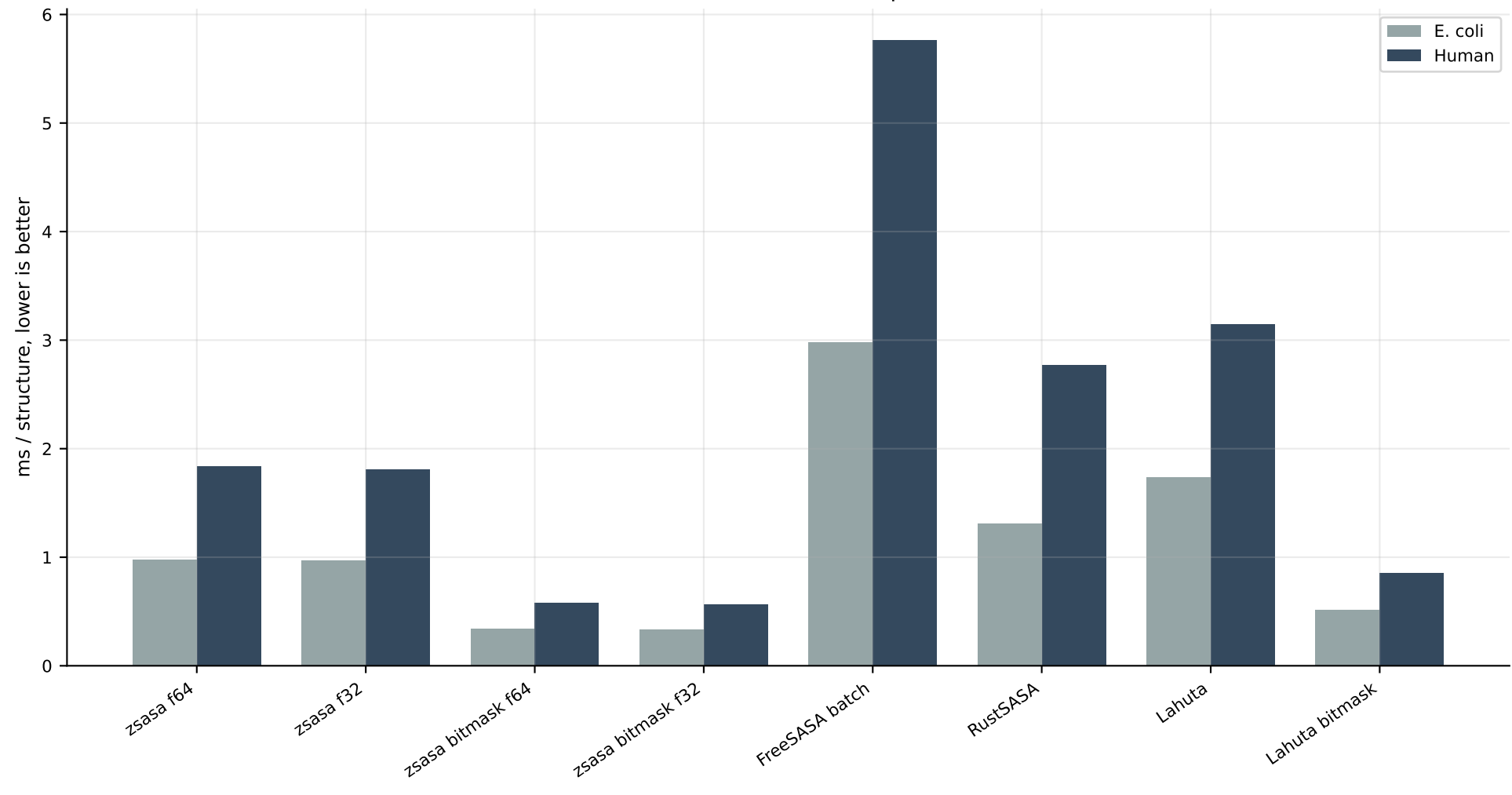
10-thread normalized runtime per structure
