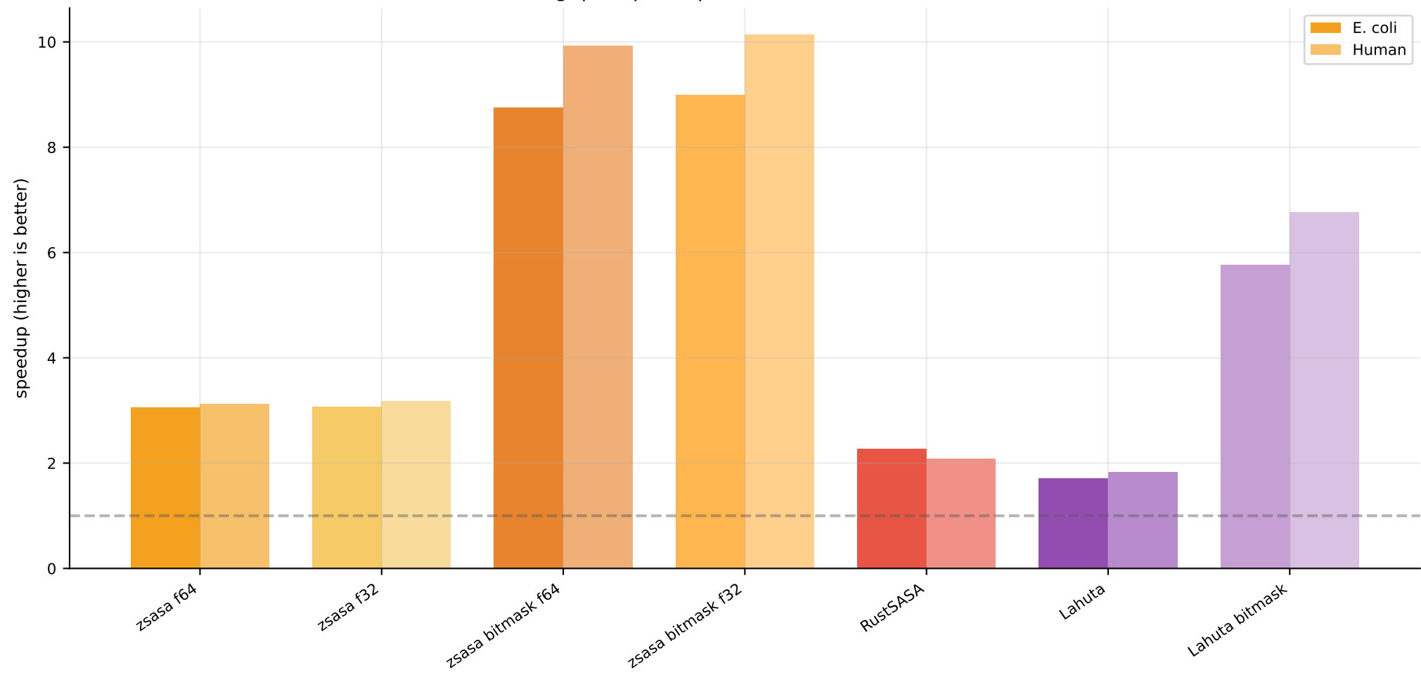
Batch throughput speedup at 10 threads vs FreeSASA batch
