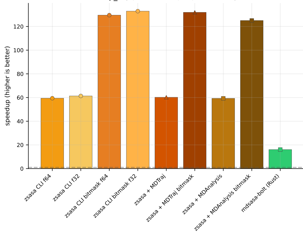
6sup_A (1,001 frames, 33,377 atoms)
