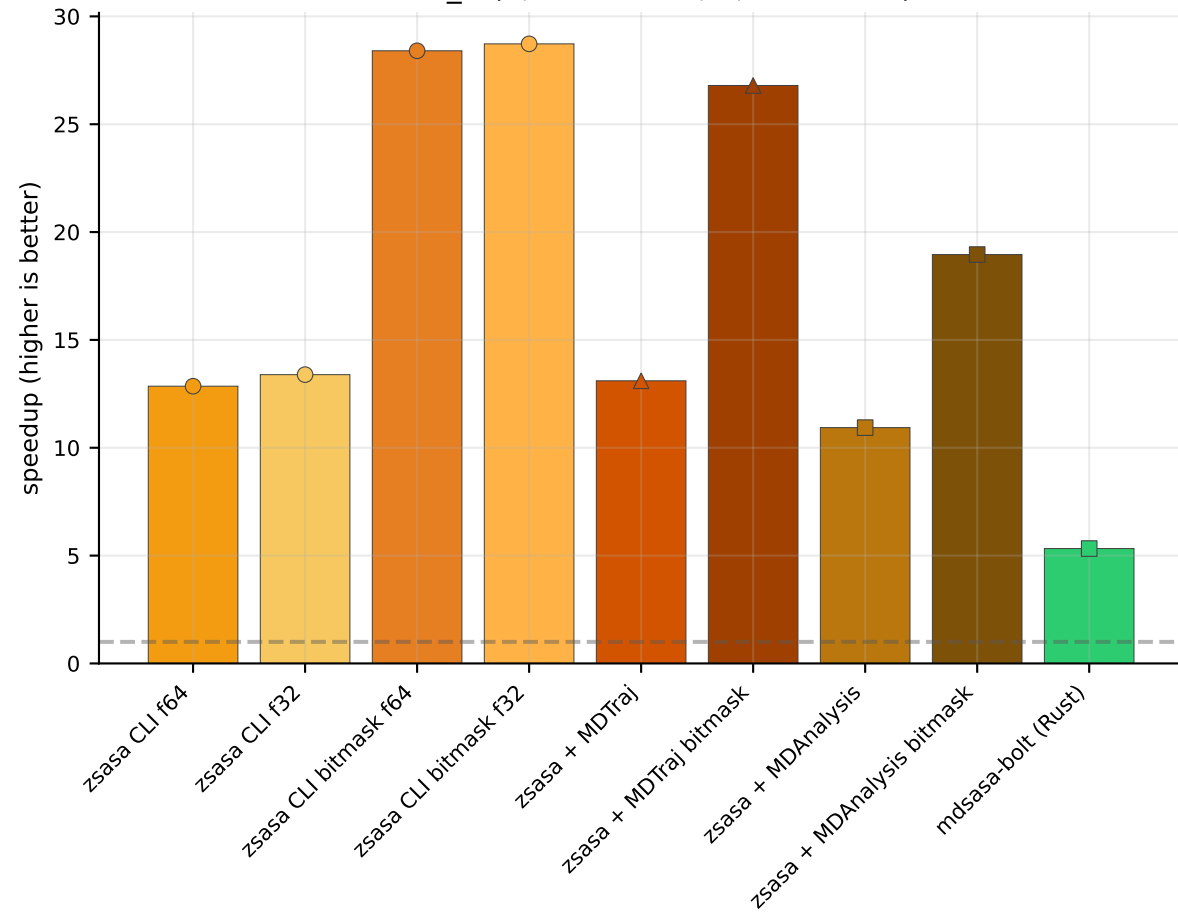
5wvo_C (1,001 frames, 3,858 atoms)
