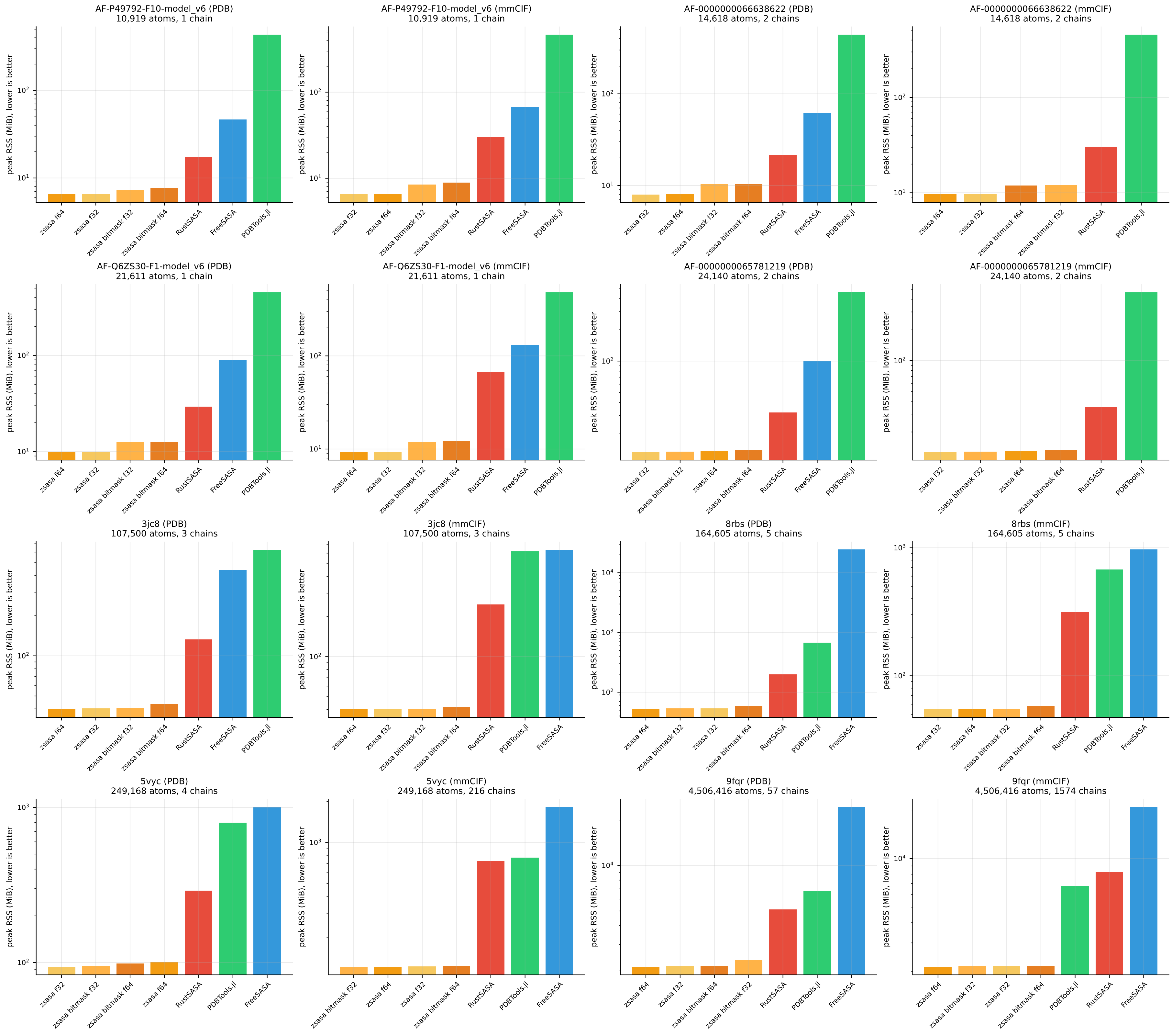
Single-file peak RSS at 10 threads
