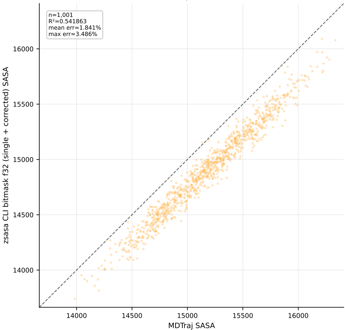
zsasa CLI bitmask f32 (single + corrected) 64 points
