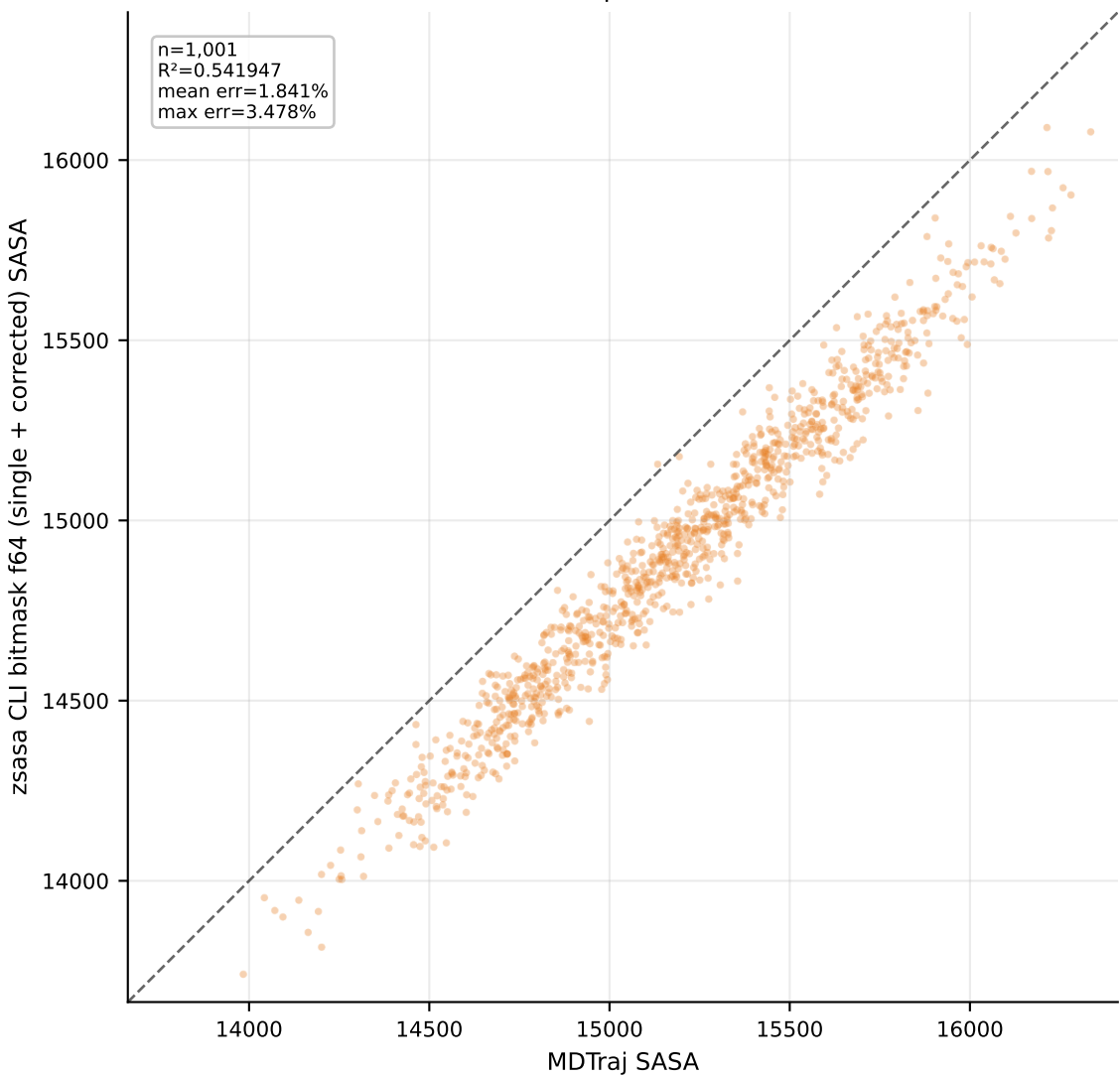
zsasa CLI bitmask f64 (single + corrected) 64 points
