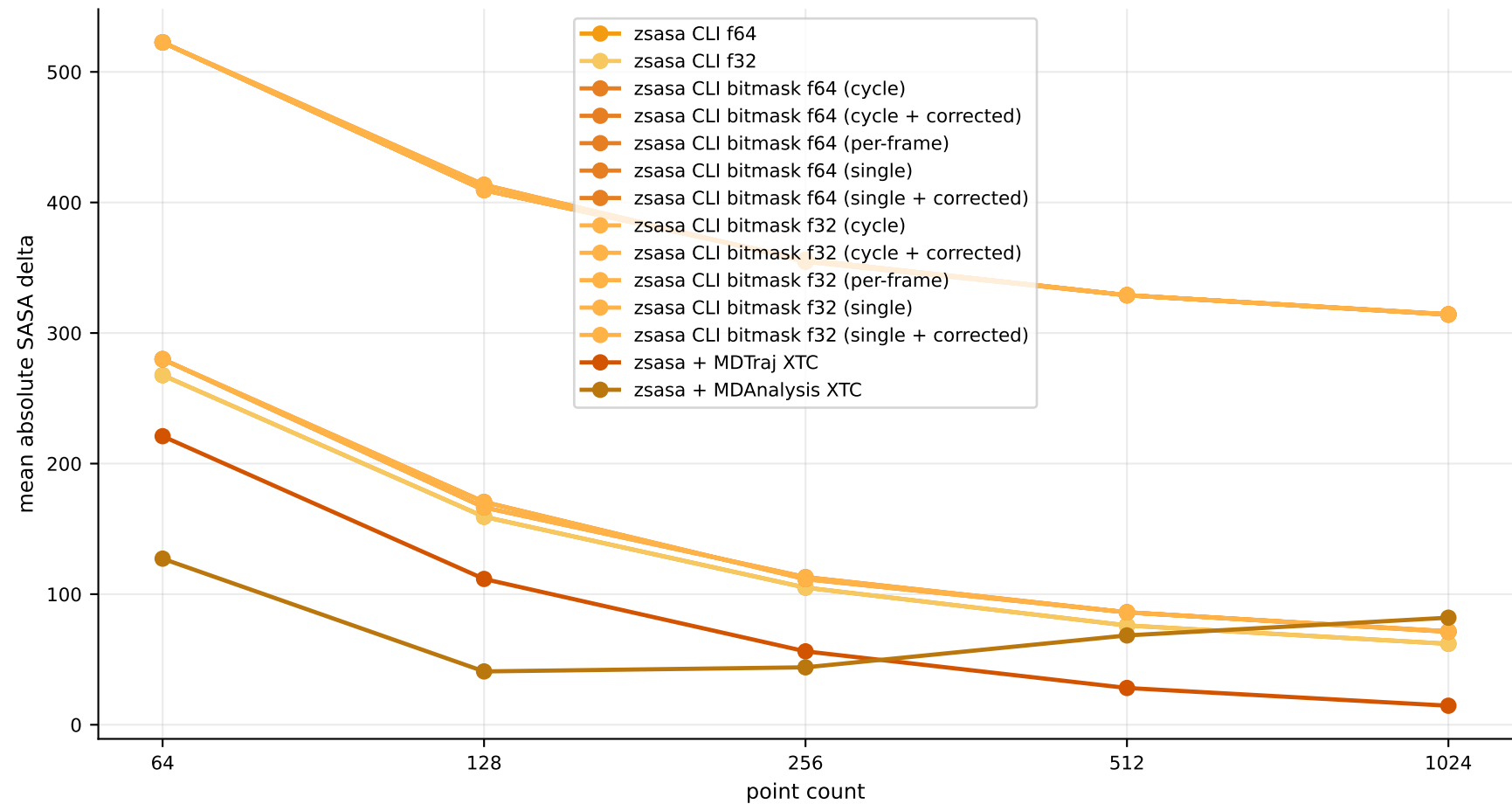
MD validation: mean absolute SASA delta
