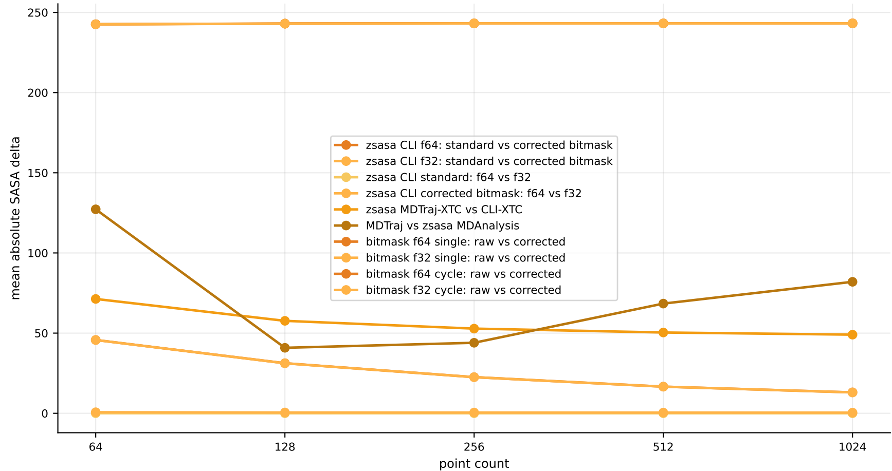
MD validation variant deltas
