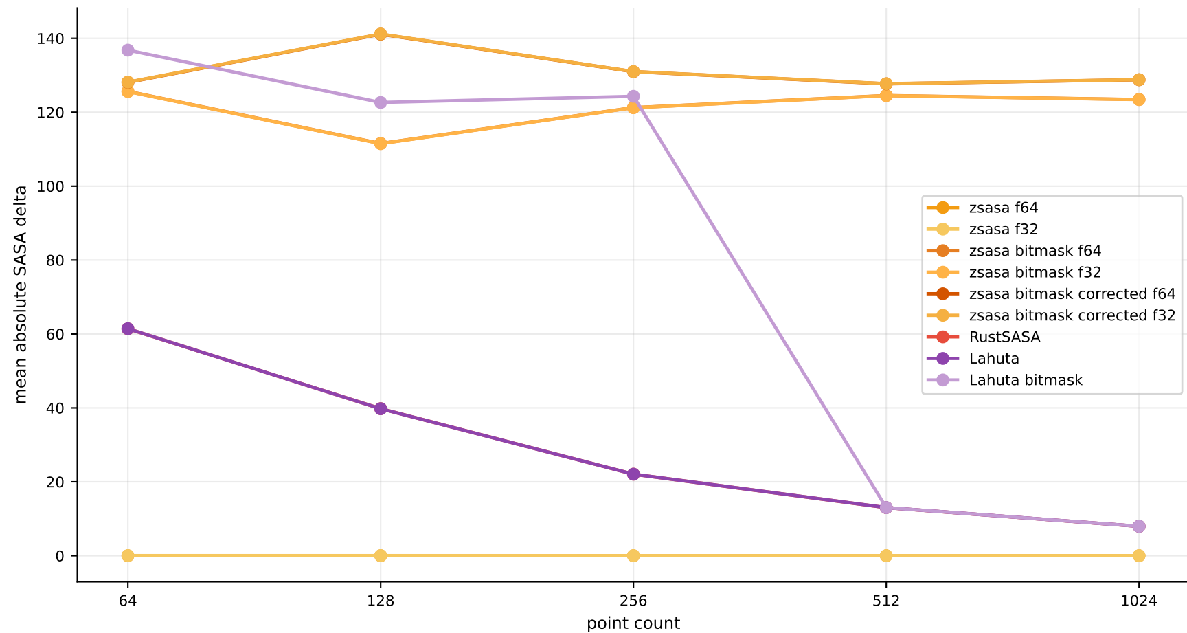
Static SR validation: mean absolute SASA delta
