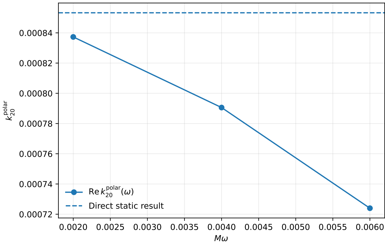
Bardeen polar near-zone response: q/q_{\text{ext}} = 0.1
