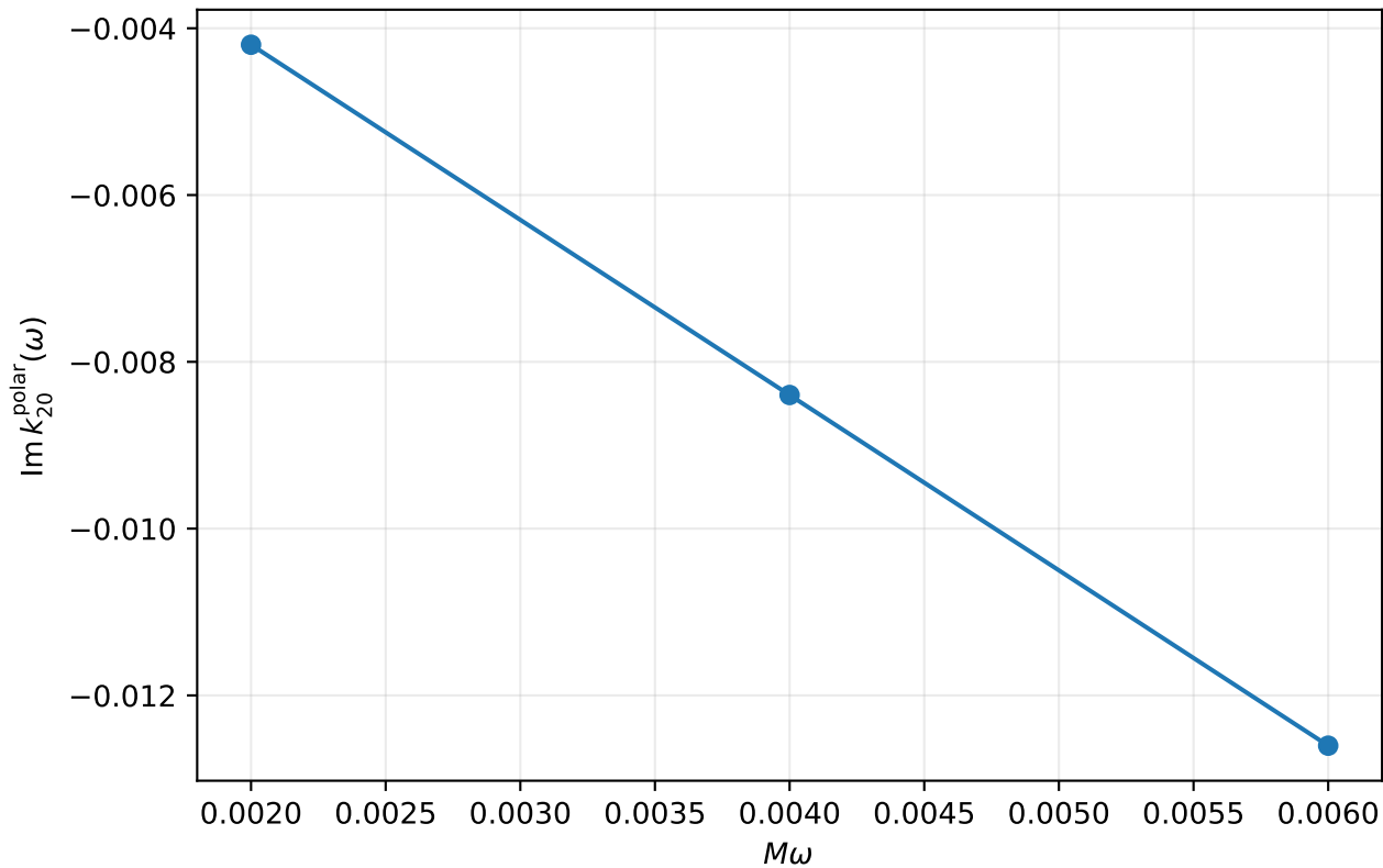
Bardeen polar dissipative response
