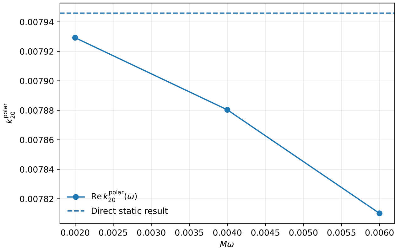
Bardeen polar near-zone response: q/q_{\text{ext}} = 0.2
