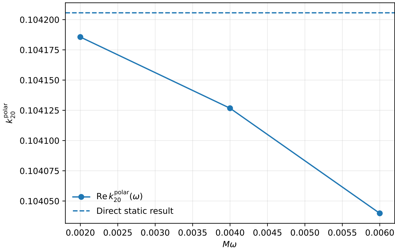
Bardeen polar near-zone response: q/q_{\text{ext}} = 0.4
