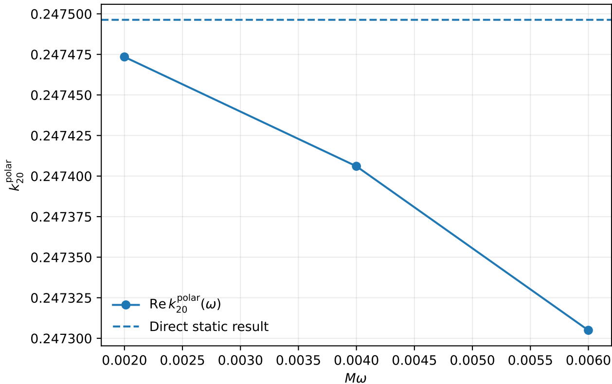
Bardeen polar near-zone response: q/q_{\text{ext}} = 0.5
