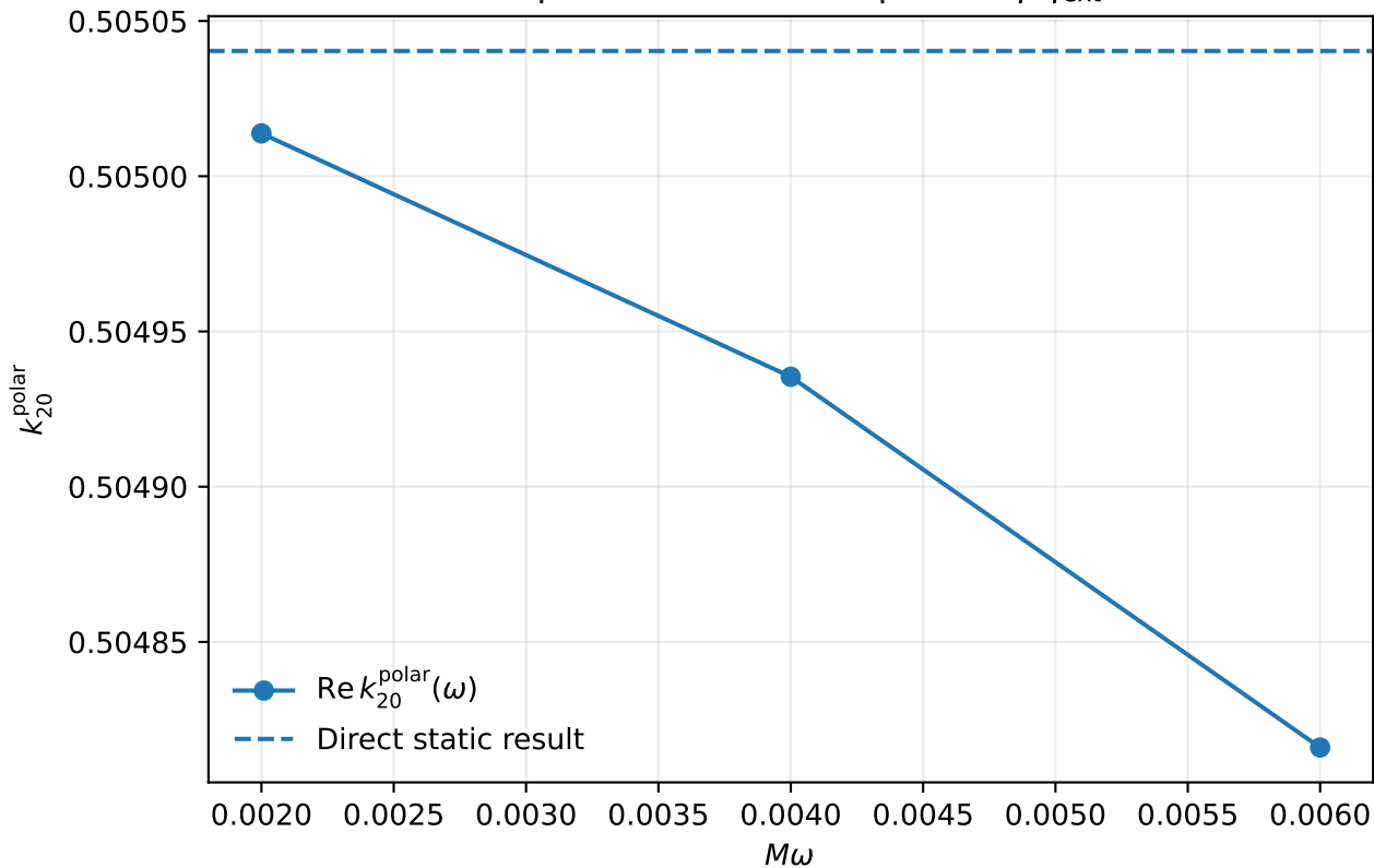
Bardeen polar near-zone response: q/q_{\text{ext}} = 0.6
