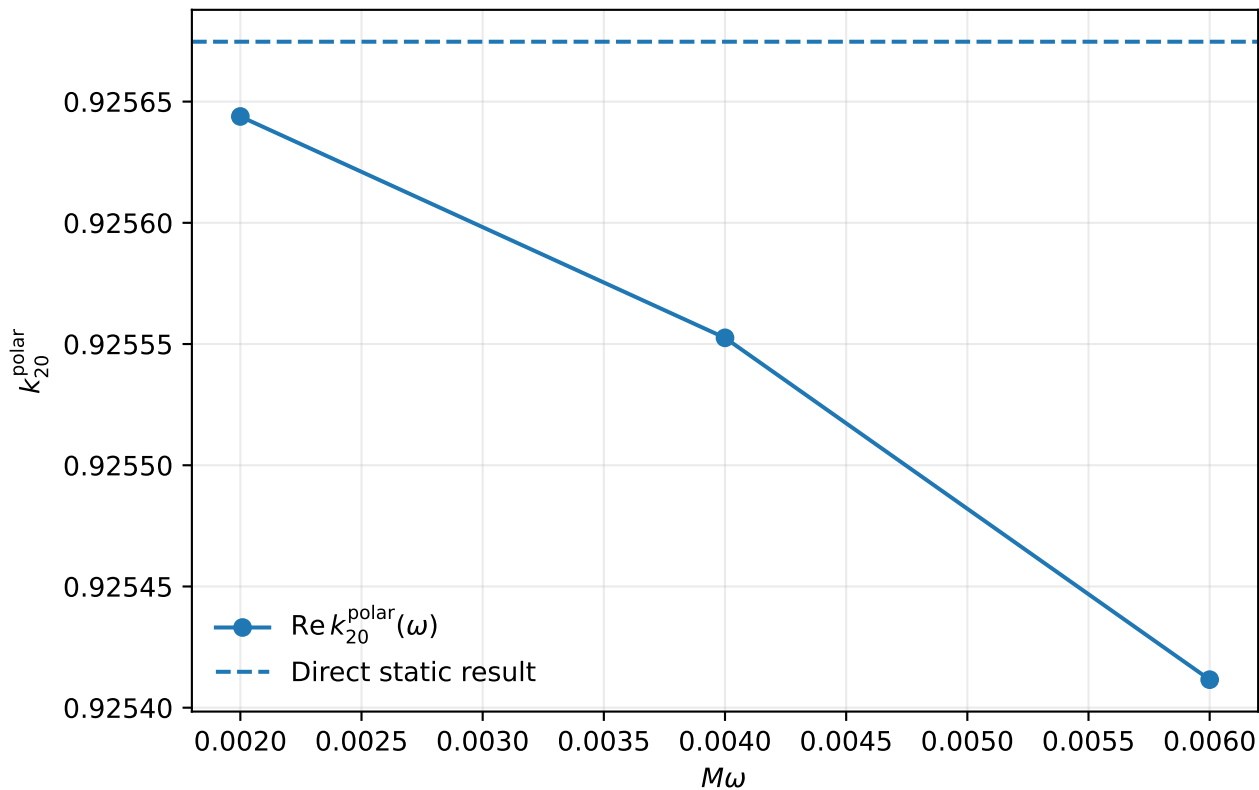
Bardeen polar near-zone response: q/q_{\text{ext}} = 0.7
