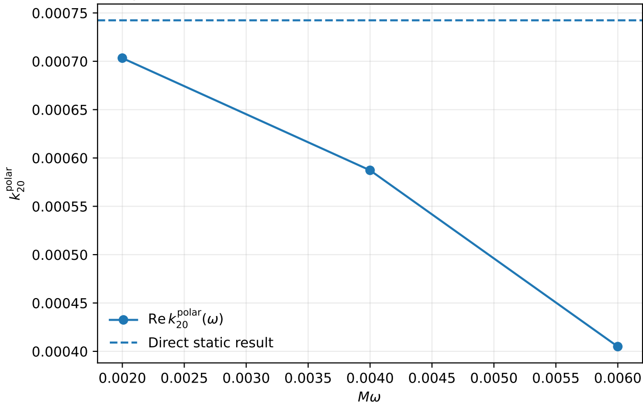
+2.491 Bardeen polar near-zone response: q/q_{\text{ext}} = 0.9
