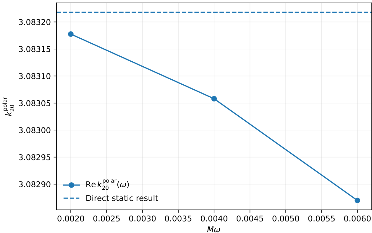
Bardeen polar near-zone response: q/q_{\text{ext}} = 0.95
