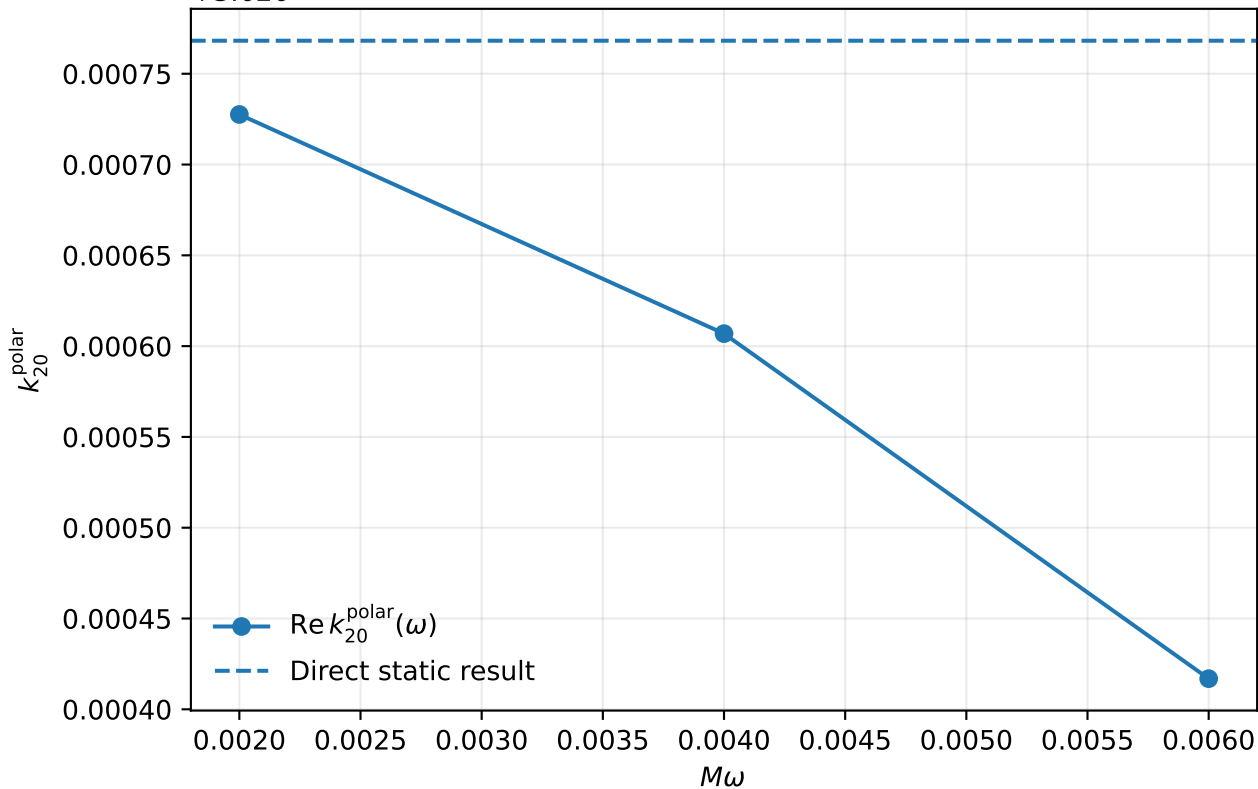
+3.626 Bardeen polar near-zone response: q/q_{\text{ext}} = 0.99
