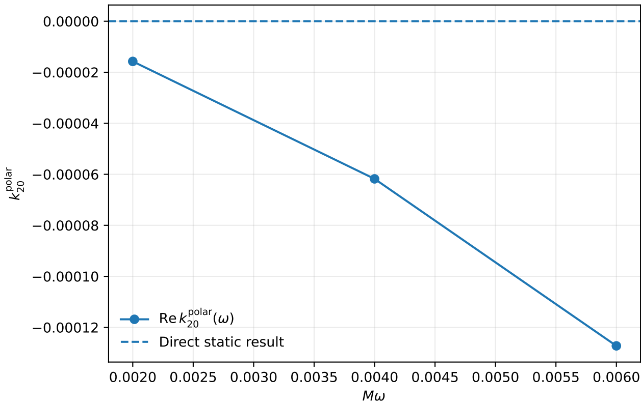
Bardeen polar near-zone response: q/q_{\text{ext}} = 1e - 05
